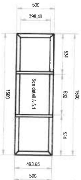
BOTTOM VIEW
