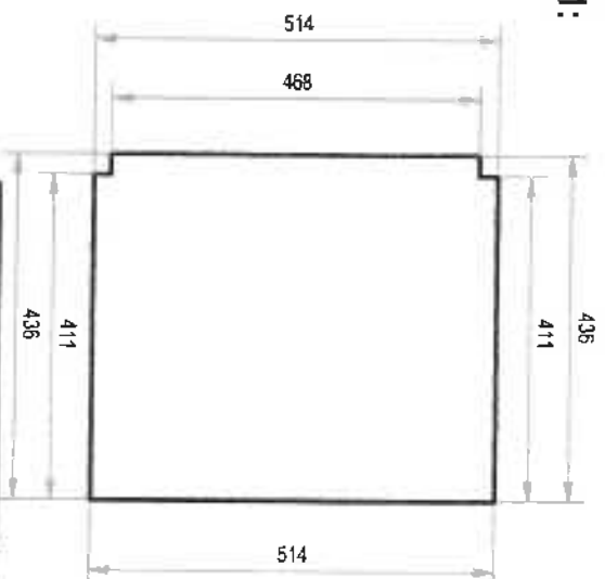
DETAIL D-1.1:
