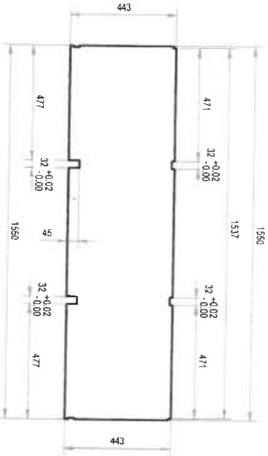
DETAIL A-5.2:
