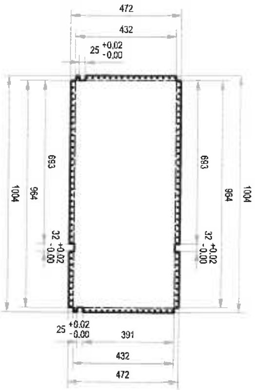
DETAIL A-3.2:
