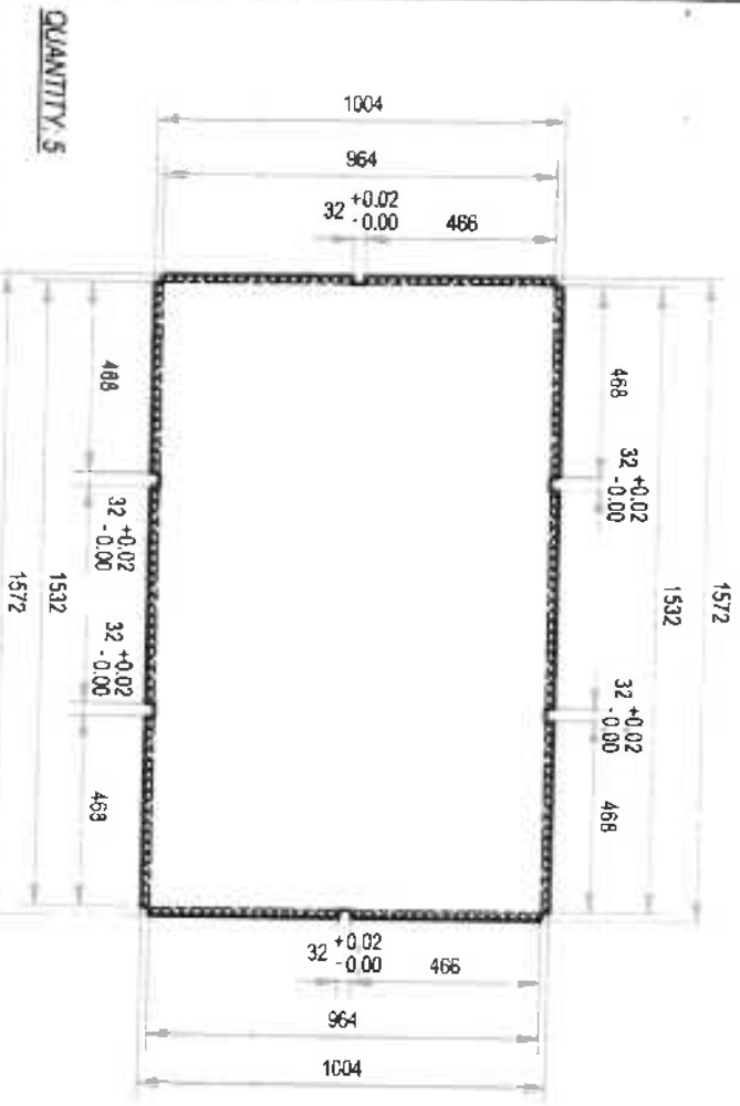
DETAIL A-2.2:
