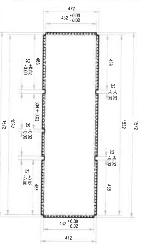
DETAIL A-1.2:
