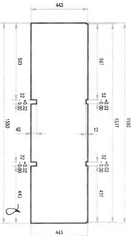
DETAIL A-5.4:
