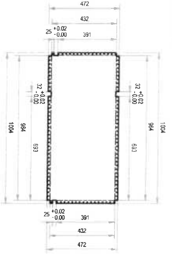
DETAIL A-4.1:
