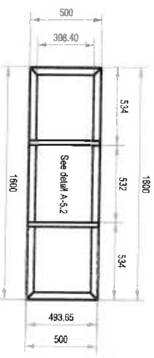
BOTTOM VIEW
