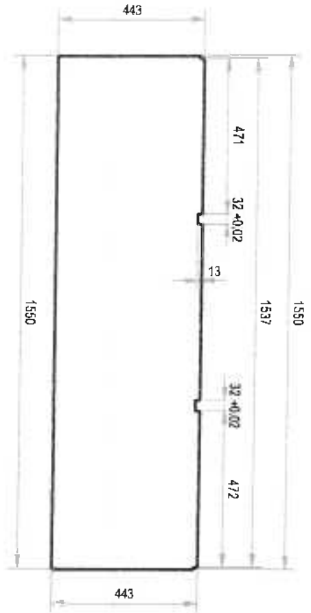
DETAIL A-5.1:
