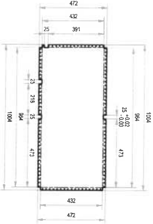
DETAIL A-4.2:
