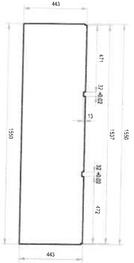
DETAIL A-5.1:
