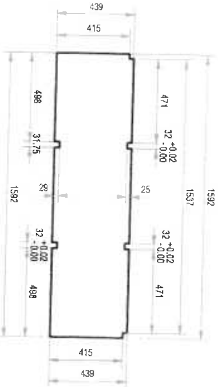
DETAIL B-1.2:
