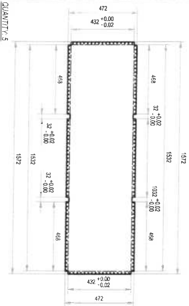
DETAIL A-1.1:
