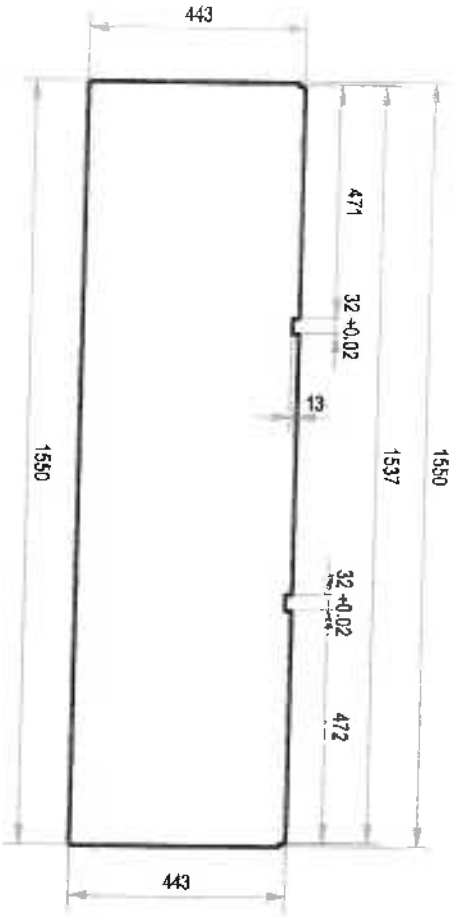
DETAIL A-5.1:
