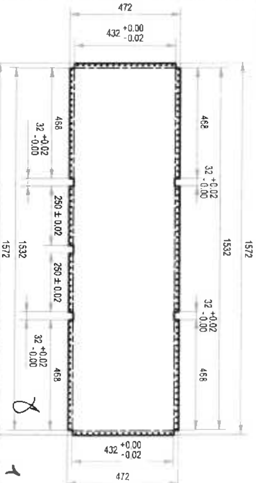
DETAIL A-1.4:
