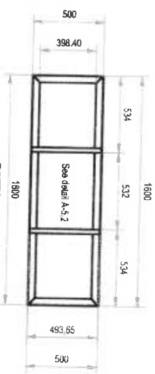
BOTTOM VIEW
