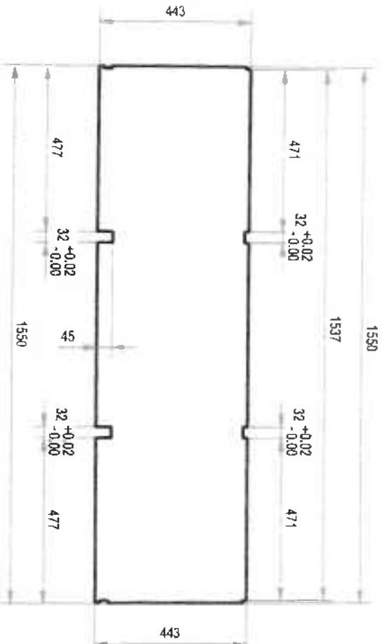
DETAIL A-5.2:
