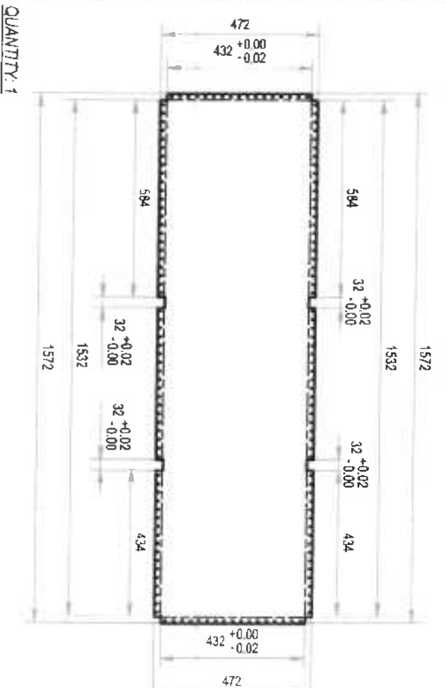
DETAIL A-1.3:
