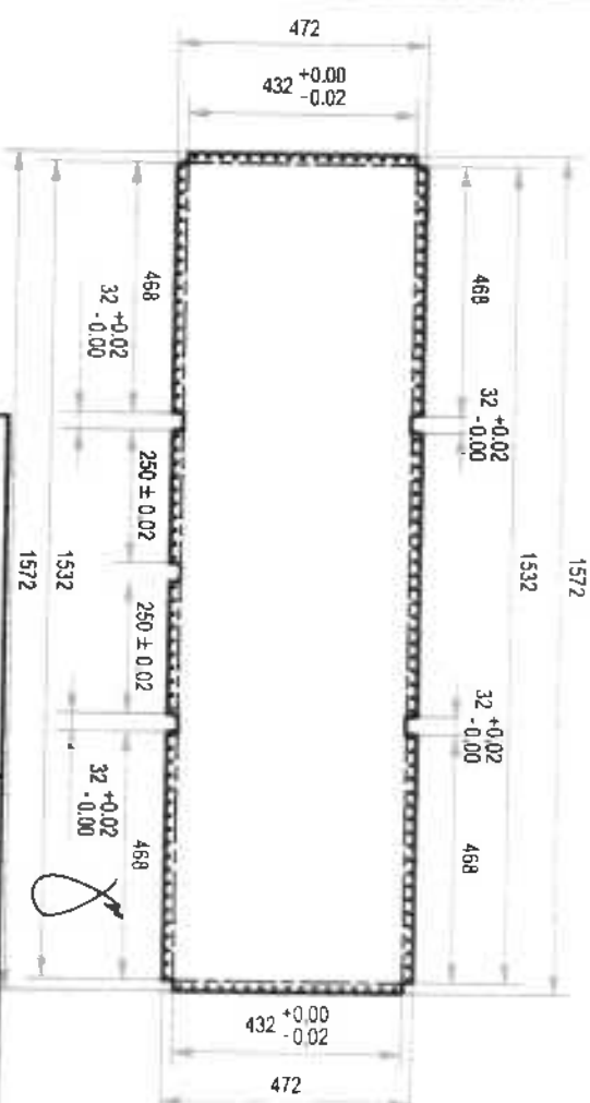
DETAIL A-1.4:
