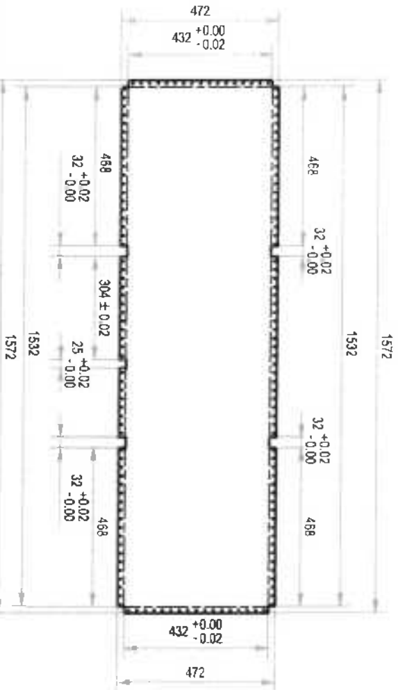
DETAIL A-1.2:
