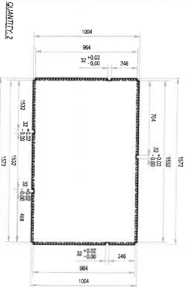
DETAIL A-2.3:
