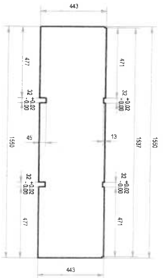
DETAIL A-5.3:
