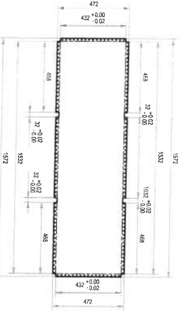
DETAIL A-1.1:
