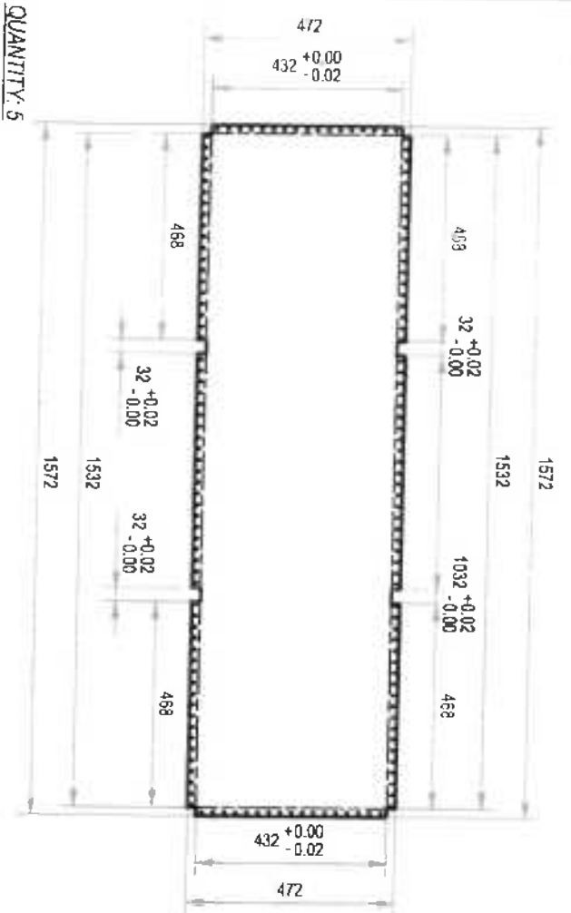
DETAIL A-1.1:
