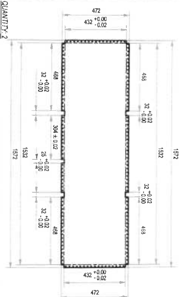
DETAIL A-1.2:
