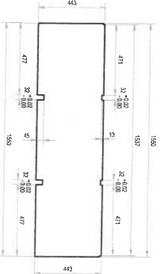
DETAIL A-5.3:
