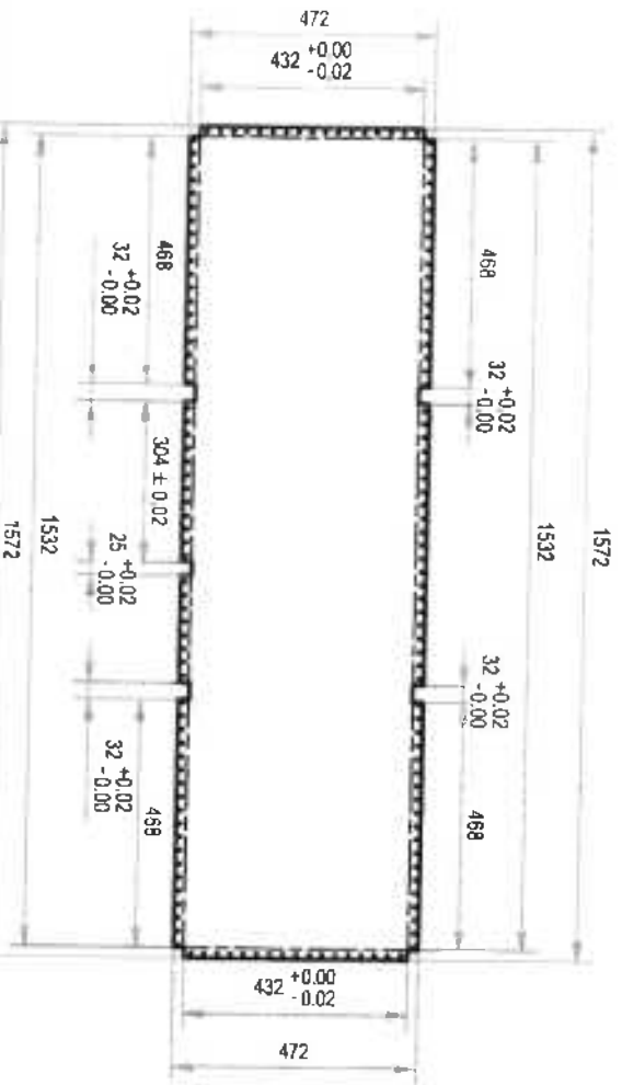
DETAIL A-1.2:
