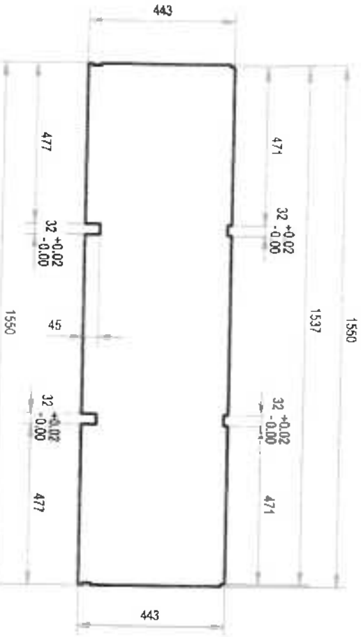
DETAIL A-5.2:
