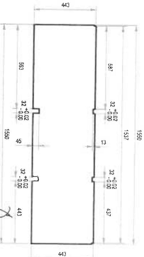
DETAIL A-5.4:
