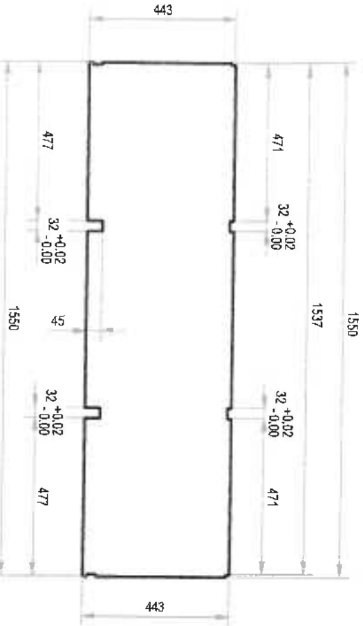
DETAIL A-5.2:
