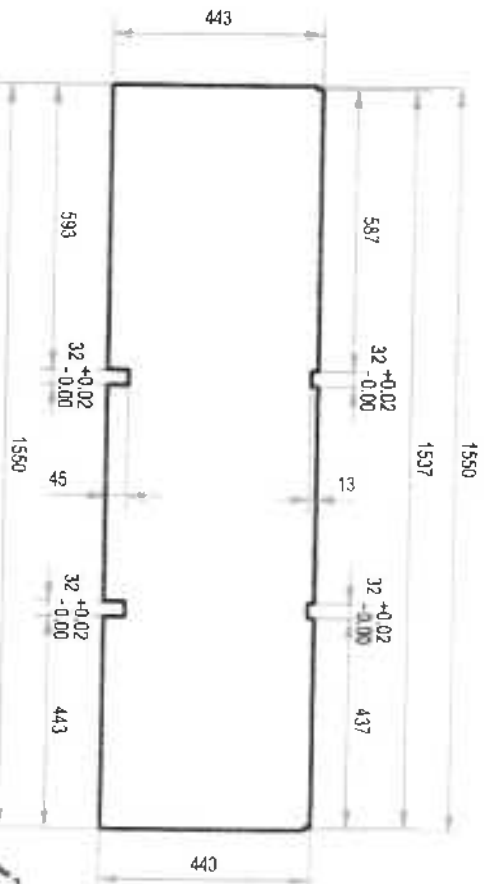
DETAIL A-5.4:
