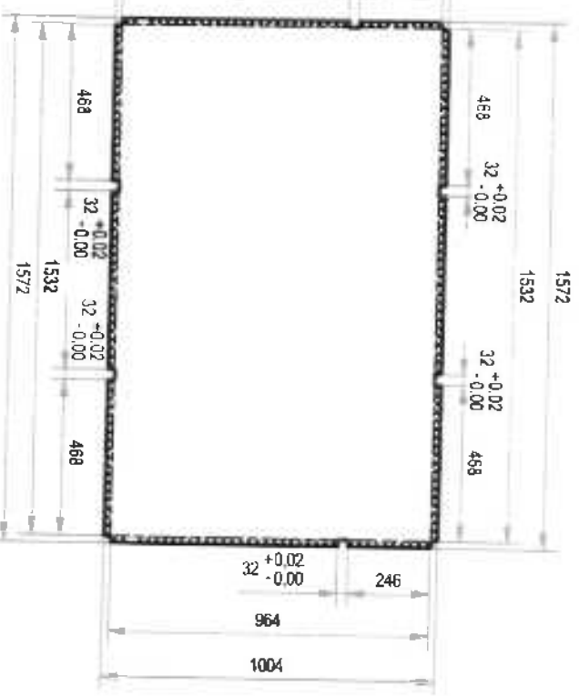
DETAIL A-2.4:
