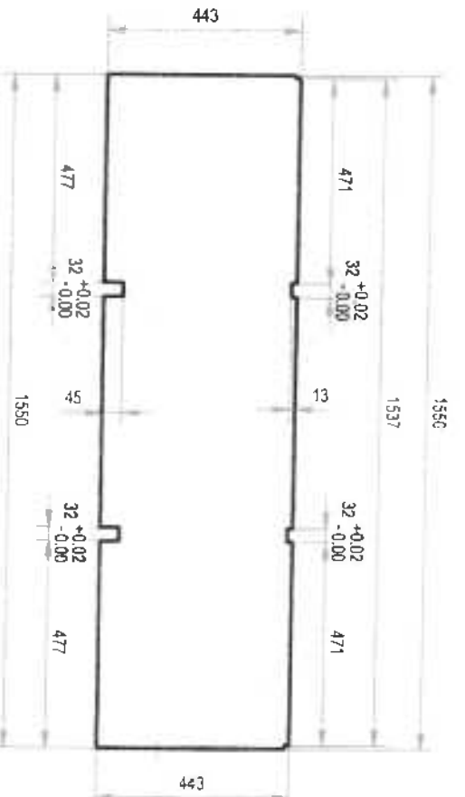
DETAIL A-5.3:
