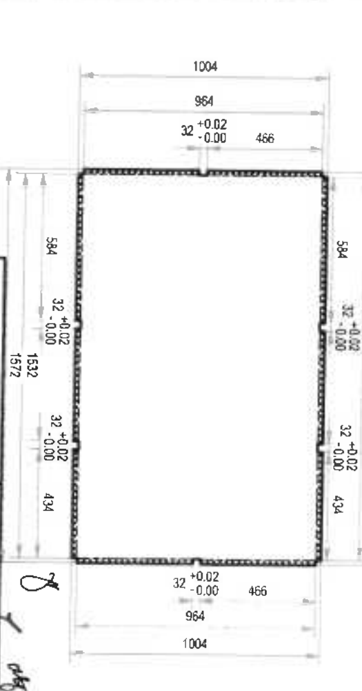
DETAIL A-2.4:
