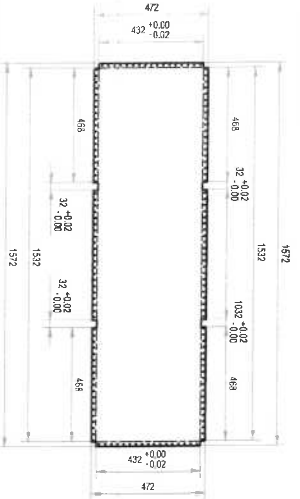
DETAIL A-1.1:
