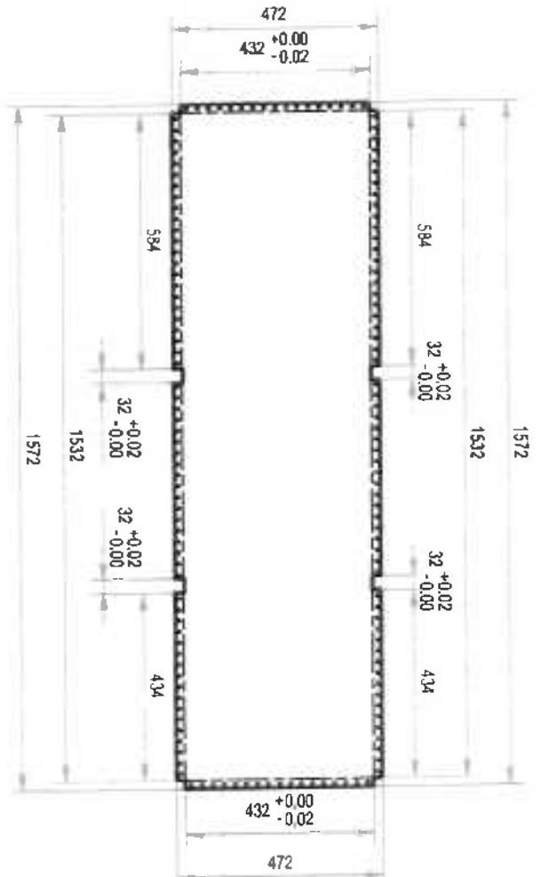
DETAIL A-1.3:
