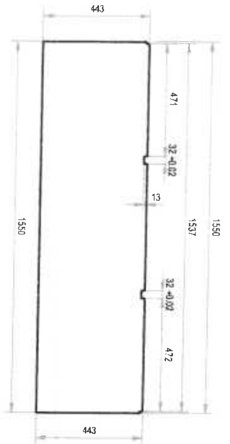
DETAIL A-5.1:
