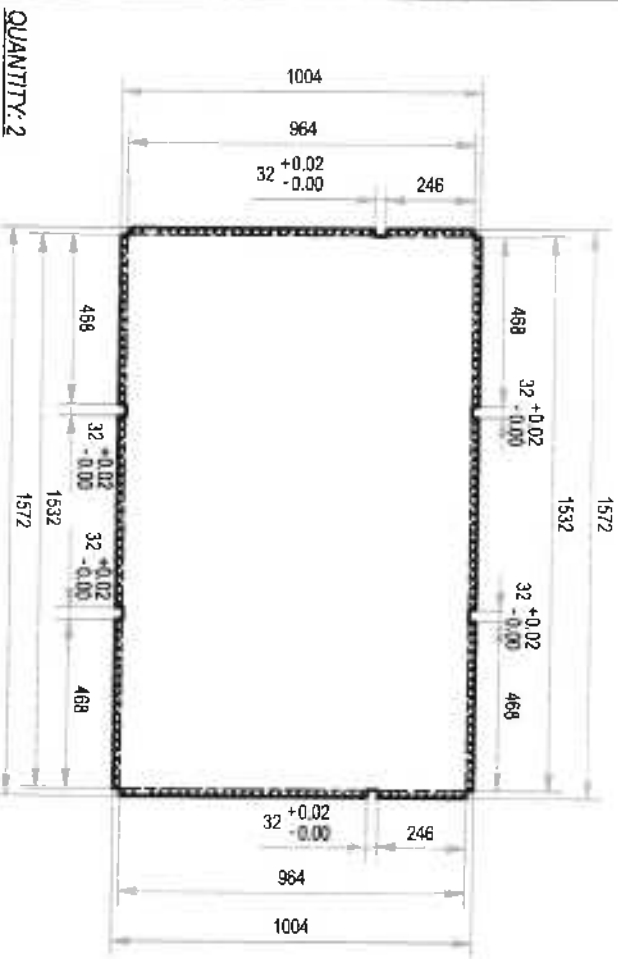
DETAIL A-2.2:
