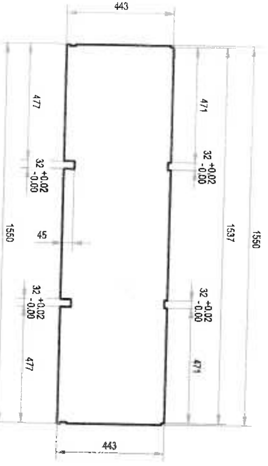
DETAIL A-5.2:
