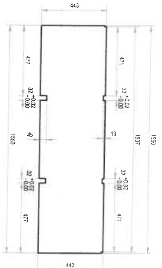
DETAIL A-5.3:
