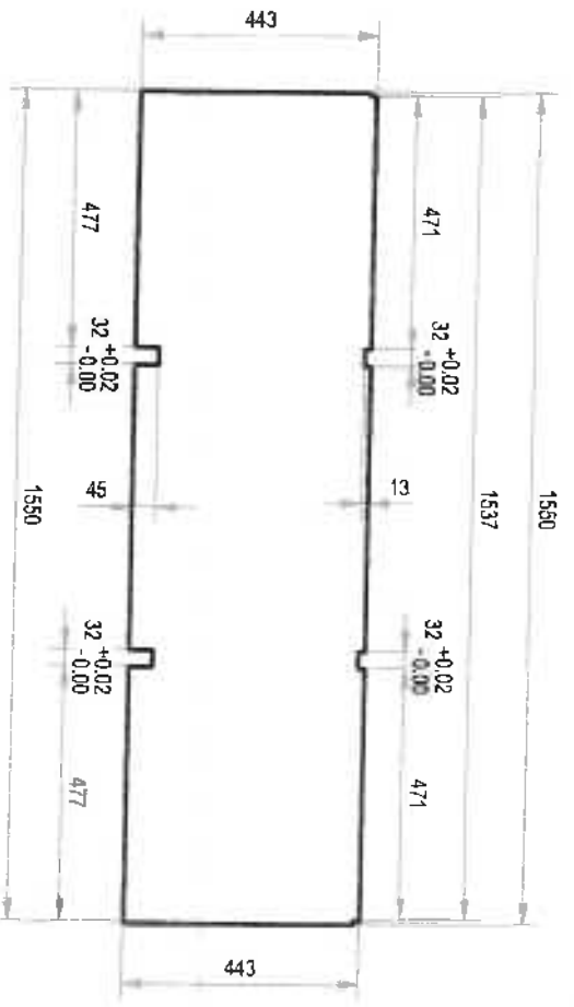
DETAIL A-5.3:
