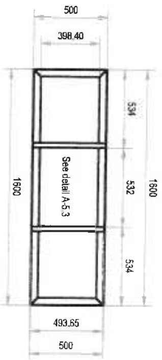
BOTTOM VIEW
