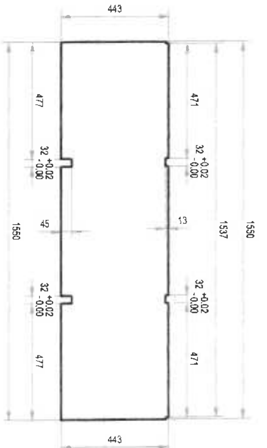
DETAIL A-5.3:
