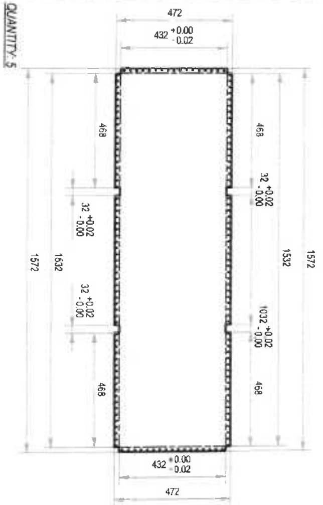
DETAIL A-1.3:
