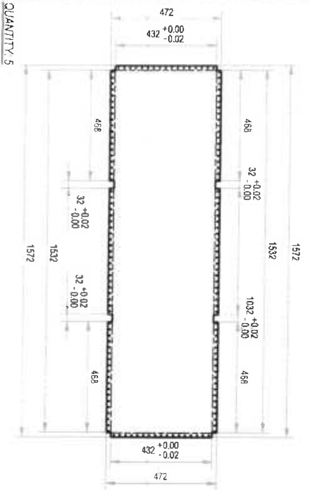
DETAIL A-1.1:
