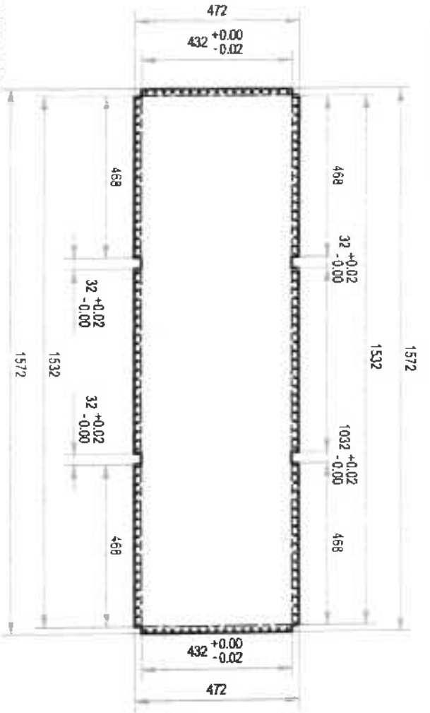
DETAIL A-1.1:
