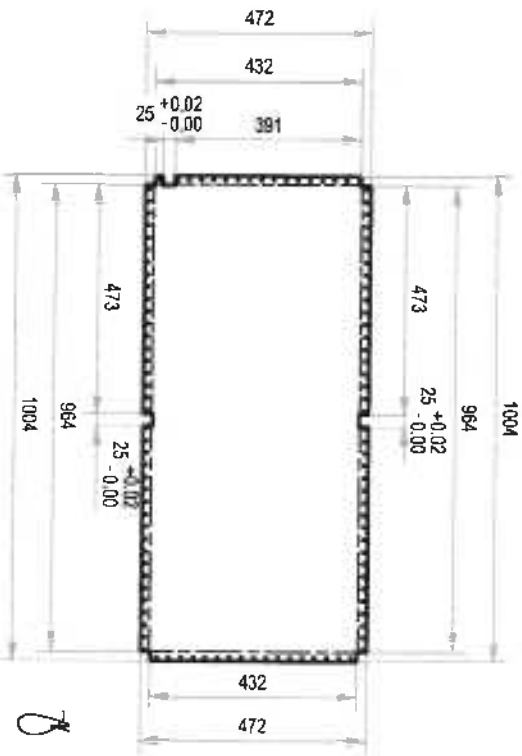
DETAIL A-3.4:
