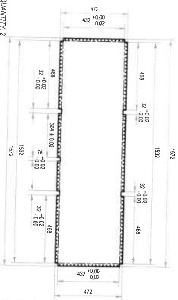
DETAIL A-1.2:
