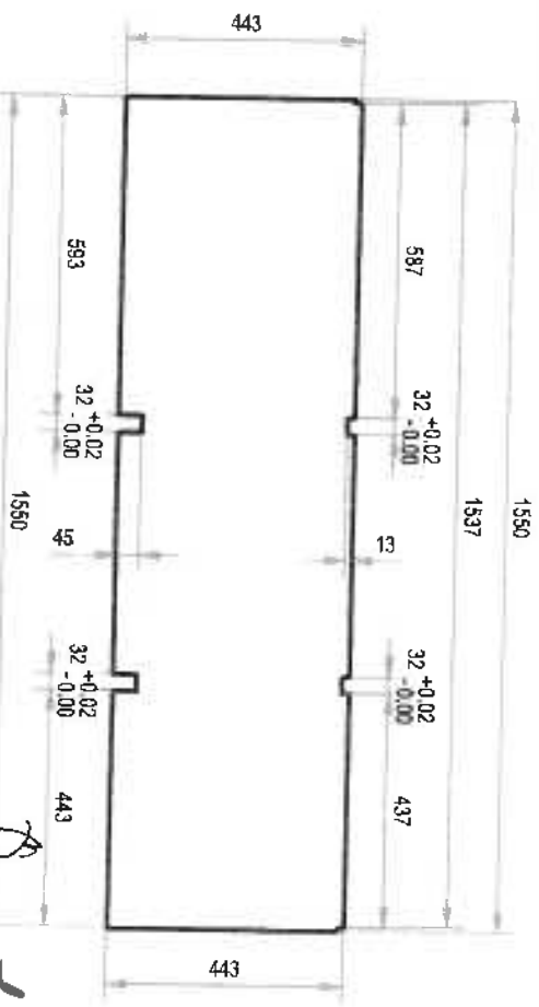
DETAIL A-5.4:
